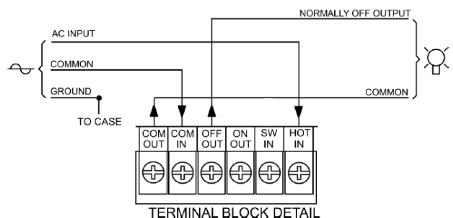
Diagram 4. SWITCHED LOADS
